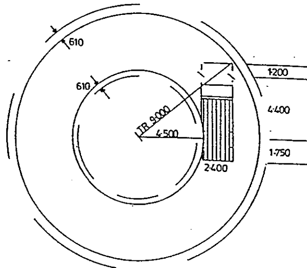
90 PERCENTILE DESIGN TWO AXLED TRUCK
