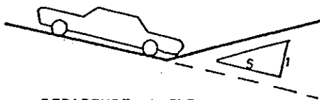
DEPARTURE ANGLE 1 in 5 max
