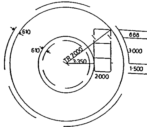
99 PERCENTILE DESIGN CAR
