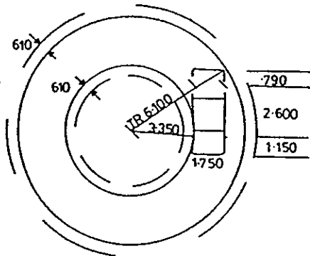
90 PERCENTILE DESIGN CAR
