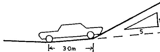
ACCESS DRIVE GRADE CHANGE 1 in 5 max at 3.0m in from kerb or edge of carriageway if no kerb.
